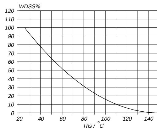
Fig.15. Normalised avalanche energy rating. W_{DSS}\% = f(T_{hs}) ; conditions: I_D = 11\text{ A}
