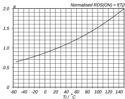
Fig.9. Normalised drain-source on-state resistance. a = R_{DS(ON)}/R_{DS(ON)25^\circ\text{C}} = f(T_j) ; I_D = 5.5 A; V_{GS} = 10 V
