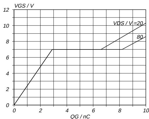
Fig.13. Typical turn-on gate-charge characteristics. V_{GS} = f(Q_G) ; conditions: I_D = 11\text{ A} ; parameter V_{DS}
