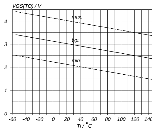
Fig.10. Gate threshold voltage. V_{GS(TO)} = f(T_j) ; conditions: I_D = 1 mA; V_{DS} = V_{GS}
