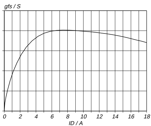
Fig.8. Typical transconductance, T_j = 25^\circ\text{C} . g_{fs} = f(I_D) ; conditions: V_{DS} = 25 V
