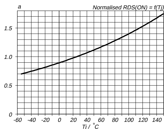
Fig.9. Normalised drain-source on-state resistance. a = R_{DS(ON)}/R_{DS(ON)25\text{ }^{\circ}\text{C}} = f(T_j) ; I_D = 8.5\text{ A} ; V_{GS} = 10\text{ V}
