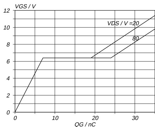
Fig.13. Typical turn-on gate-charge characteristics. V_{GS} = f(Q_G) ; conditions: I_D = 26\text{ A} ; parameter V_{DS}
