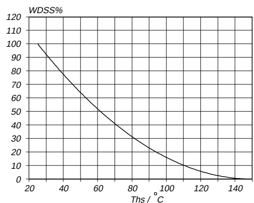
Fig.15. Normalised avalanche energy rating. W_{DSS}\% = f(T_{hs}) ; conditions: I_D = 26\text{ A}
