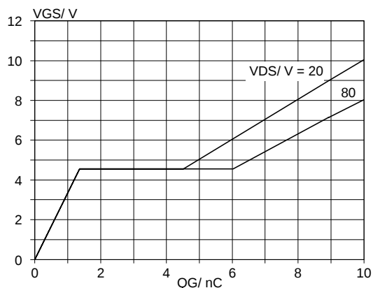
Fig.13. Typical turn-on gate-charge characteristics. V_{GS} = f(Q_G) ; conditions: I_D = 1.8\text{ A} ; parameter V_{DS}
