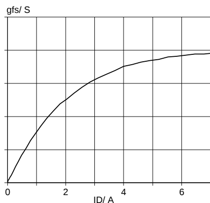
Fig. 8. Typical transconductance, T_j = 25 \text{ °C} . g_{fs} = f(I_D) ; conditions: V_{DS} = 25 \text{ V}
