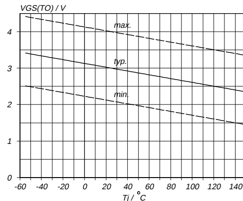
Fig. 10. Gate threshold voltage. V_{GS(TH)} = f(T_j) ; conditions: I_D = 1 \text{ mA} ; V_{DS} = V_{GS}
