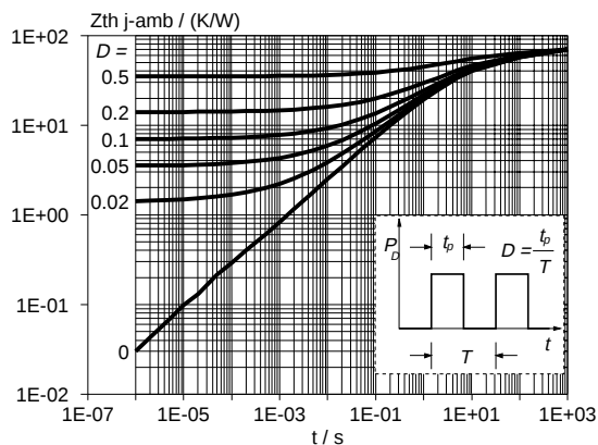
Fig.3. Transient thermal impedance. Z_{th\ j\text{-}amb} = f(t) ; parameter D = t_p / T
