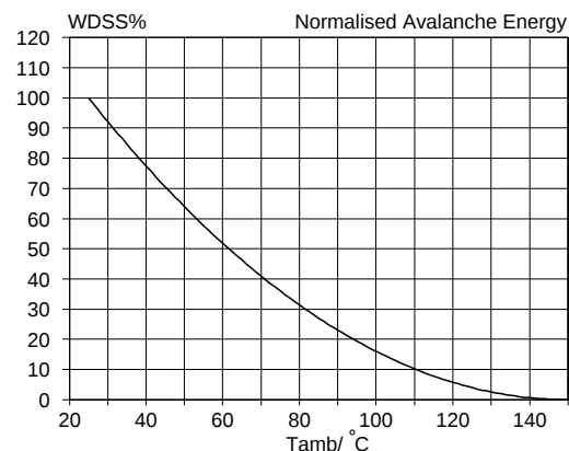
Fig.15. Normalised avalanche energy rating. W_{DSS}\% = f(T_{amb}) ; conditions: I_D = 1.8\text{ A}
