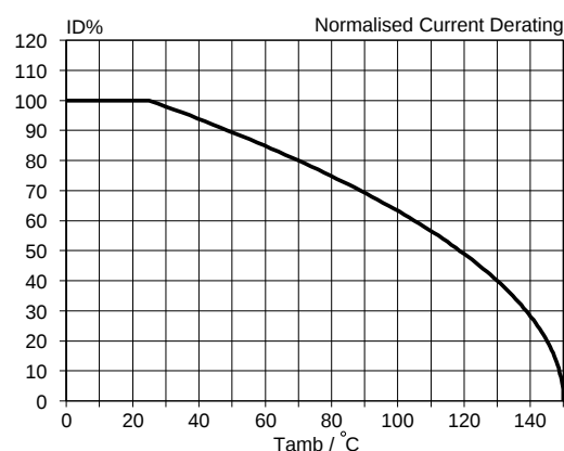
Fig.2. Normalised continuous drain current. ID\% = 100 \cdot I_D / I_{D\ 25^\circ\text{C}} = f(T_{\text{amb}}) ; conditions: V_{GS} \geq 10\text{ V}
