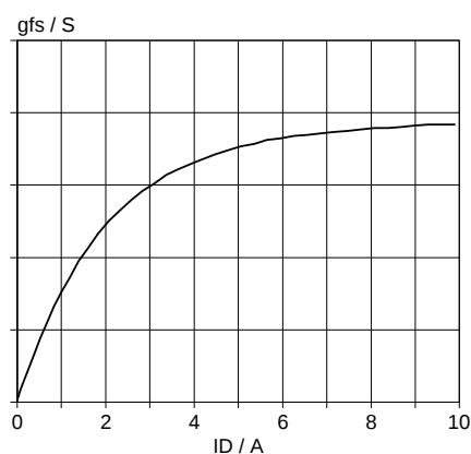
Fig.8. Typical transconductance, T_J = 25^\circ \text{C} . g_{fs} = f(I_D) ; conditions: V_{DS} = 25 \text{ V}
