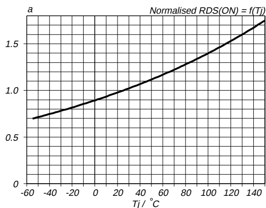
Fig.9. Normalised drain-source on-state resistance. a = R_{DS(ON)} / R_{DS(ON)25^\circ \text{C}} = f(T_J) ; I_D = 2.7 \text{ A} ; V_{GS} = 10 \text{ V}
