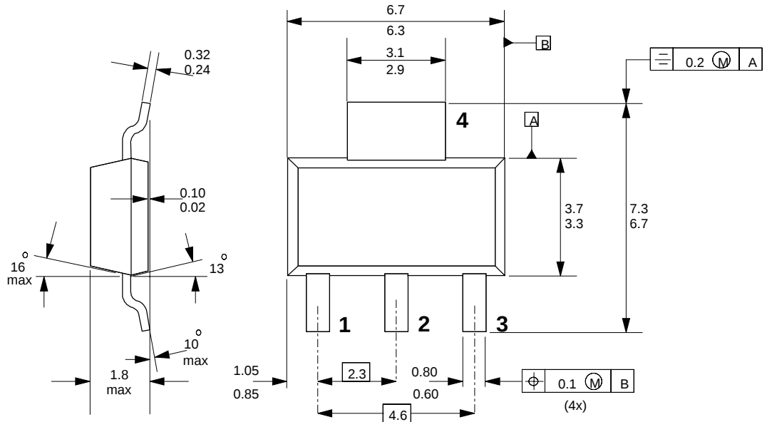
Fig.19. SOT223 surface mounting package.
