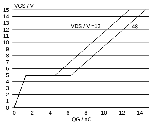
Fig.13. Typical turn-on gate-charge characteristics. V_{GS} = f(Q_G) ; conditions: I_D = 2.7 A; parameter V_{DS}
