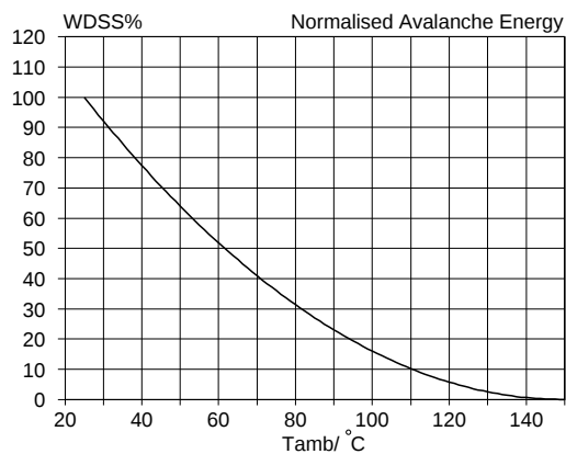
Fig.15. Normalised avalanche energy rating. W_{DSS}\% = f(T_{amb}) ; conditions: I_D = 2.7 A
