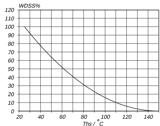
Fig.15. Normalised avalanche energy rating. W_{DSS}\% = f(T_{hs}) ; conditions: I_D = 13\text{ A}
