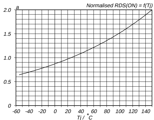
Fig. 9. Normalised drain-source on-state resistance. a = R_{DS(ON)}/R_{DS(ON)25\text{ }^{\circ}\text{C}} = f(T_j) ; I_D = 5\text{ A} ; V_{GS} = 5\text{ V}
