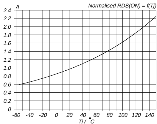
Fig. 9. Normalised drain-source on-state resistance. a = R_{DS(ON)}/R_{DS(ON)25\text{ }^{\circ}\text{C}} = f(T_j) ; I_D = 7\text{ A} ; V_{GS} = 5\text{ V}
