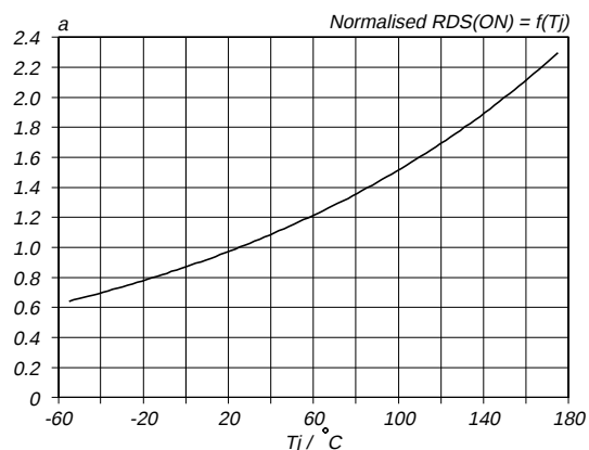
Fig.9. Normalised drain-source on-state resistance. a = R_{DS(ON)}/R_{DS(ON)25^\circ C} = f(T_J) ; I_D = 5.5 A; V_{GS} = 5 V
