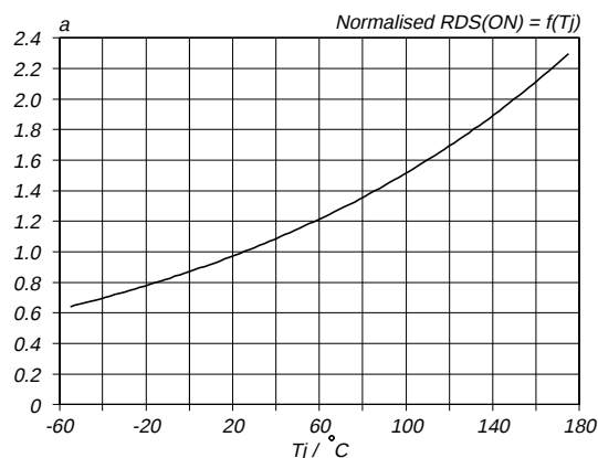
Fig.9. Normalised drain-source on-state resistance. a = R_{DS(ON)}/R_{DS(ON)25^\circ \text{C}} = f(T_j) ; I_D = 13 \text{ A} ; V_{GS} = 5 \text{ V}
