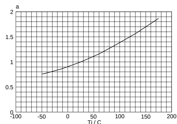
Fig.10. Normalised drain-source on-state resistance. a = R_{DS(ON)}/R_{DS(ON)25^\circ\text{C}} = f(T_j) ; I_D = 25\text{ A} ; V_{GS} = 5\text{ V}
