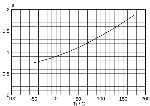
Fig. 9. Normalised drain-source on-state resistance. a = R_{DS(ON)}/R_{DS(ON)25\text{ °C}} = f(T_j) ; I_D = 25 A; V_{GS} = 10 V
