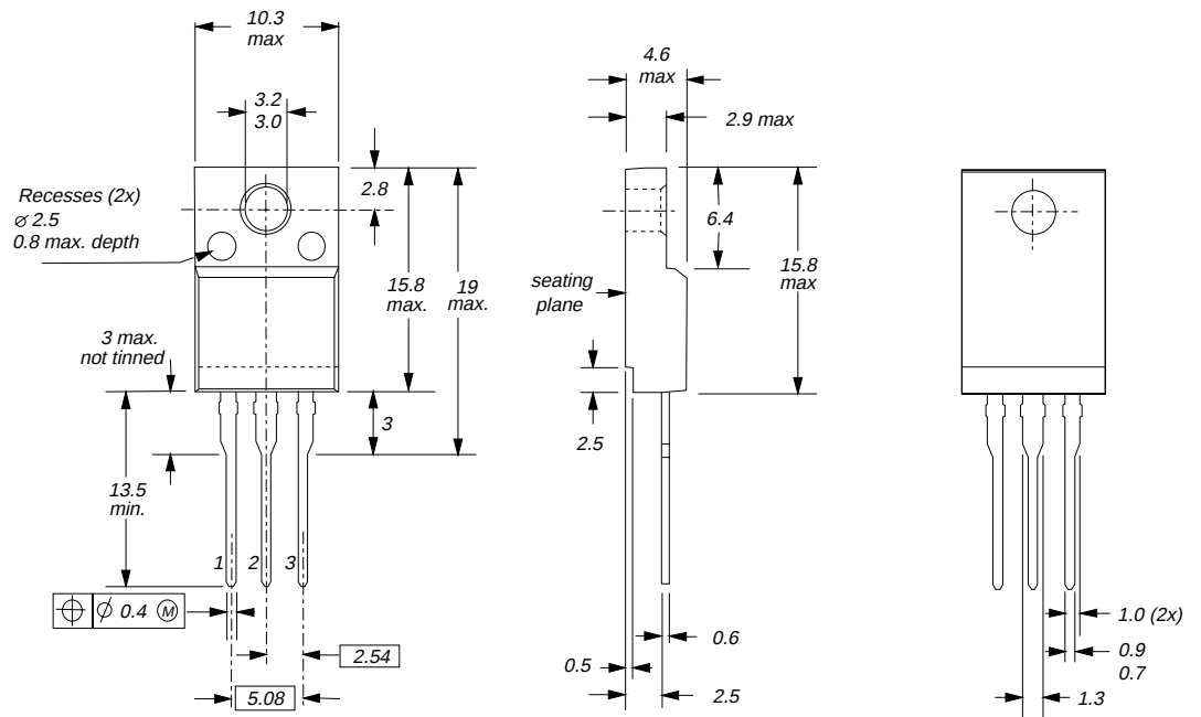
Fig.18. SOT186A; The seating plane is electrically isolated from all terminals.
