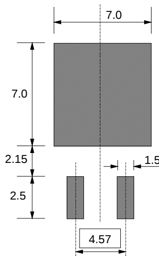
Fig.2. SOT428 : soldering pattern for surface mounting.
