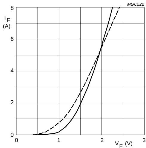
BYD33D to M Solid line: T_j = 25^\circ\text{C} . Dotted line: T_j = 175^\circ\text{C} .
