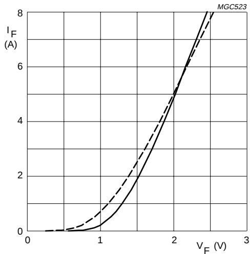
BYD33U and V Solid line: T_j = 25^\circ\text{C} . Dotted line: T_j = 175^\circ\text{C} .
