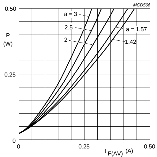
BYD71E to G a = I_{F(RMS)}/I_{F(AV)} ; V_R = V_{RRMmax} ; \delta = 0.5 .
