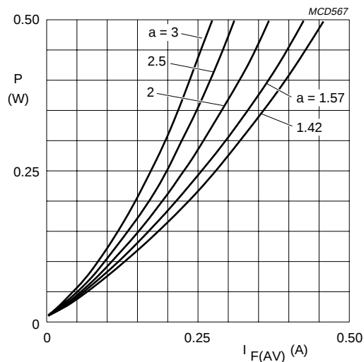
BYD71A to D a = I_{F(RMS)}/I_{F(AV)} ; V_R = V_{RRMmax} ; \delta = 0.5 .
