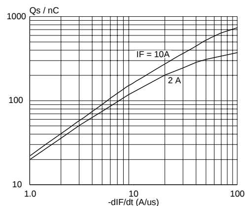
Fig.8. Maximum Q_s at T_j = 25^\circ\text{C}
