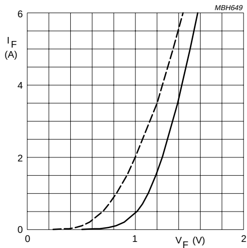
BYV27-500 and 600 Dotted line: T_j = 175^\circ\text{C} . Solid line: T_j = 25^\circ\text{C} .
