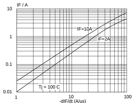
Fig. 8. Maximum I_{rms} at T_j = 100^\circ\text{C} .
