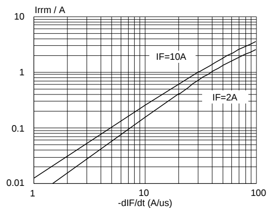
Fig. 7. Maximum I_{rms} at T_j = 25^\circ\text{C} .
