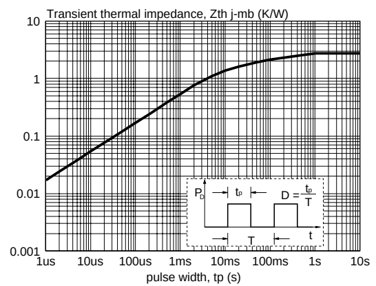
Fig.11. Transient thermal impedance; Z_{th\ j-mb} = f(t_p) .
