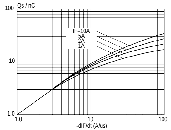
Fig.10. Maximum Q_s at T_j = 25\text{ }^{\circ}\text{C} .
