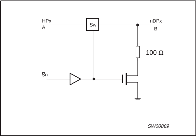
SIMPLIFIED SCHEMATIC, EACH FET SWITCH
