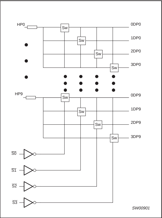
LOGIC DIAGRAM (POSITIVE LOGIC)
