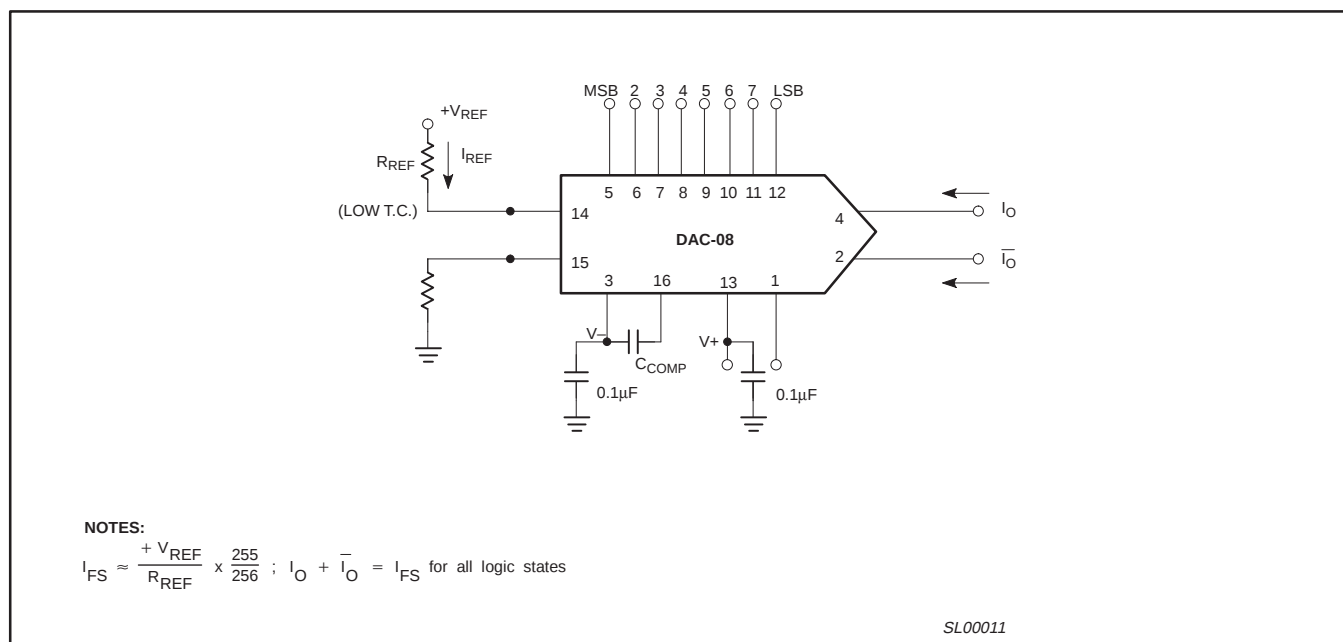
Figure 11. Basic DAC-08 Configuration
