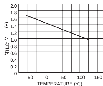
V_{TH} - V_{LC} vs Temperature
