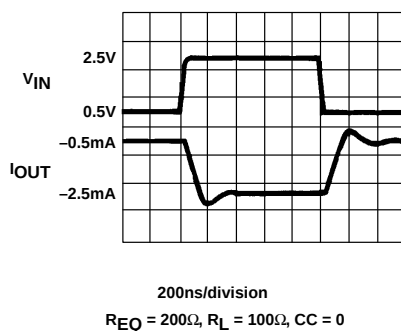
LSB Switching
