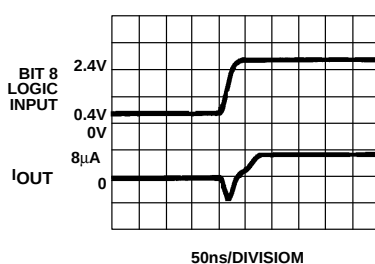
LSB Switching
