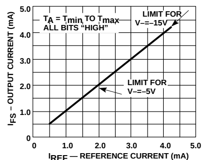
Full-Scale Current vs Reference Current
