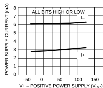
Power Supply Current vs V_+
