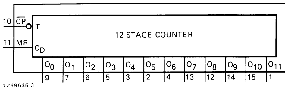
Fig.1 Functional diagram.
