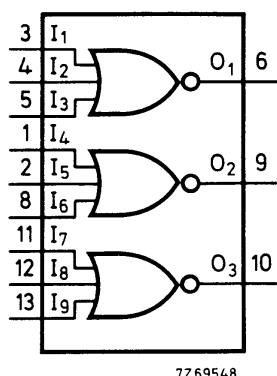
Fig.1 Functional diagram.
