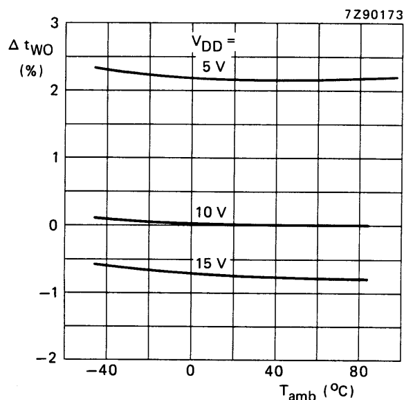
(b) R t = 100 kΩ; C t = 2 nF.
