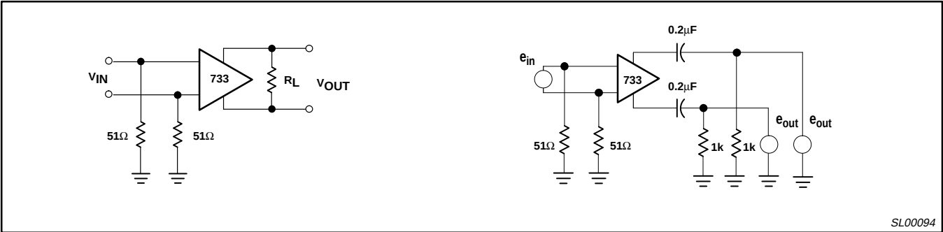
Figure 6. Test Circuits
