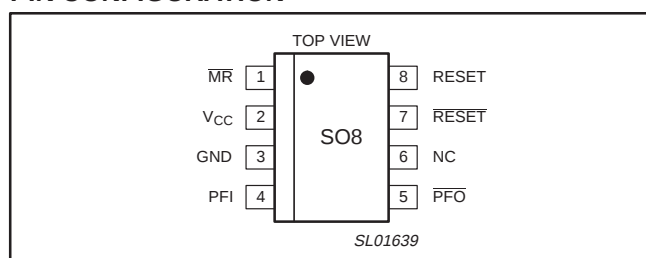
Figure 2. Pin configuration.
