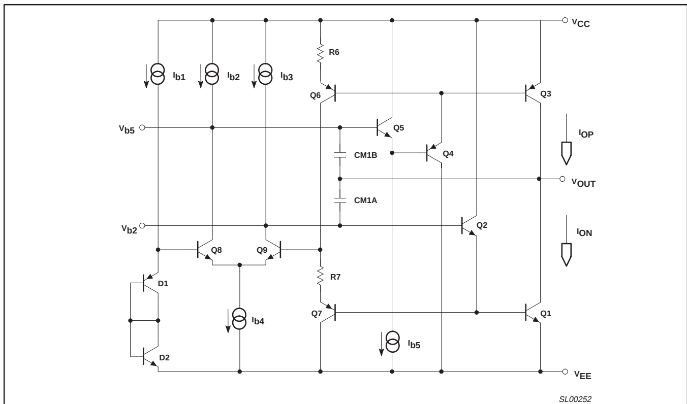
Figure 3. Output Stage
