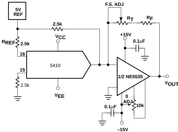
Figure 10. Bipolar Voltage Output Circuits (-10V to +10V)
