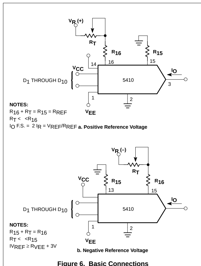
Figure 6. Basic Connections
