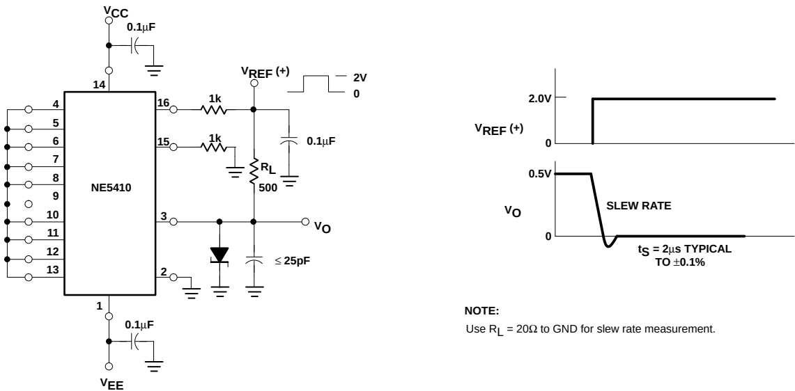
Figure 9. Reference Amplifier Settling Time and Slew Rate
