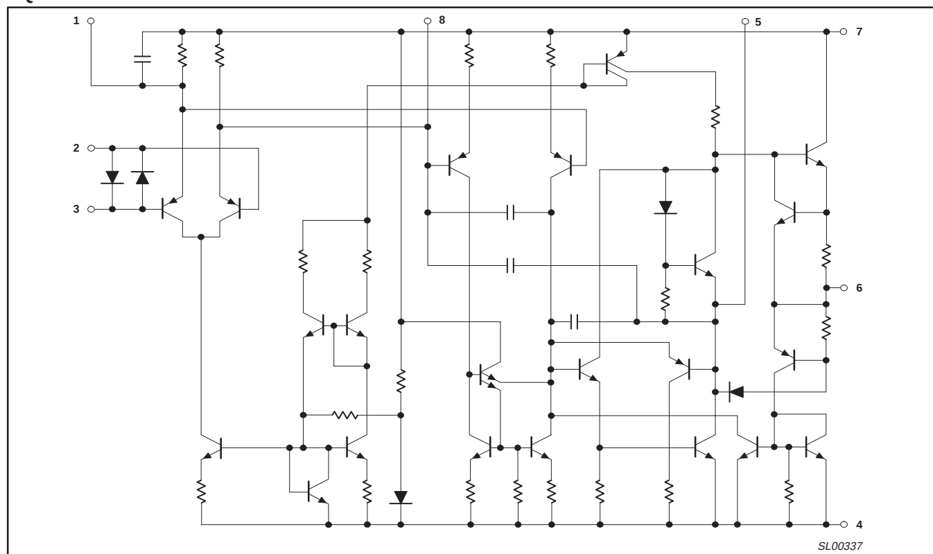
Figure 2. Equivalent Schematic
