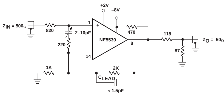
Figure 11. Non-Inverting Follower
