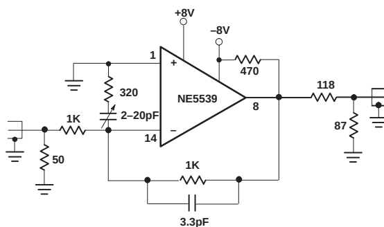
Figure 12. Inverting Follower
