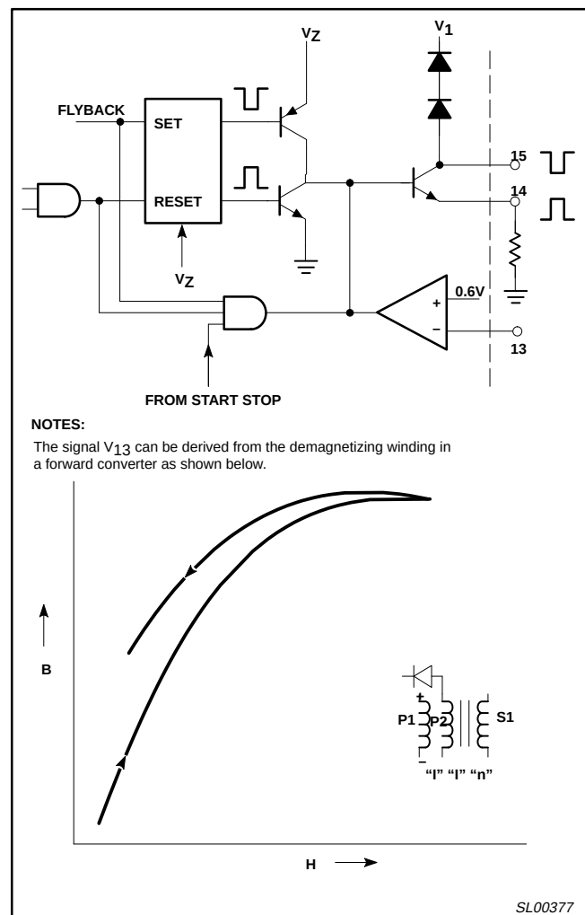
Figure 18. Output Stage
