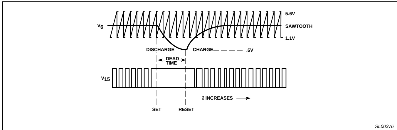
Figure 17. Start-Stop Circuit
