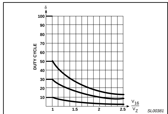
Figure 22. Feed-Forward Regulation
