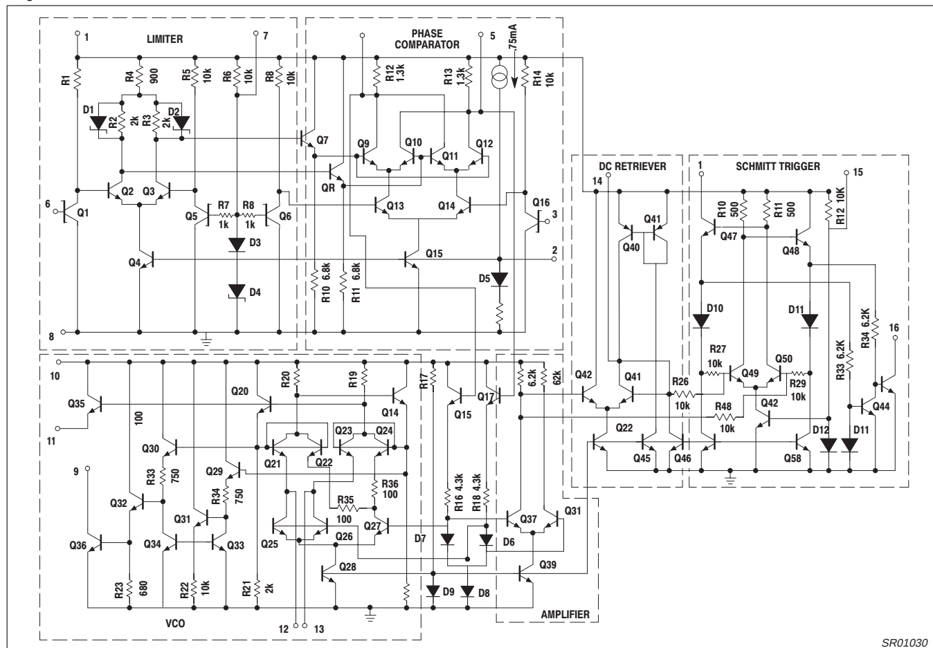
Figure 6. Equivalent Schematic
