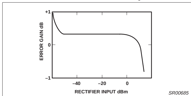
Figure 11. Rectifier Accuracy
