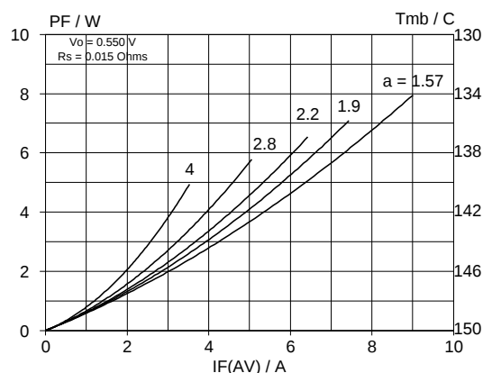
Fig.2. Maximum forward dissipation P_F = f(I_{F(AV)}) ; sinusoidal current waveform where a = form factor = I_{F(RMS)} / I_{F(AV)} .
