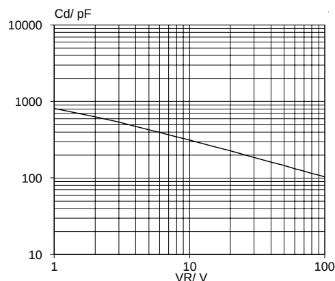
Fig.5. Typical junction capacitance; C_d = f(V_R) ; f = 1 MHz; T_j = 25 C to 125 C.
