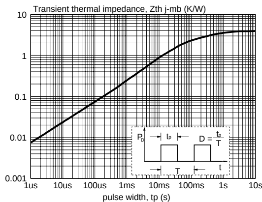
Fig.6. Transient thermal impedance; Z_{th j-mb} = f(t_p) .
