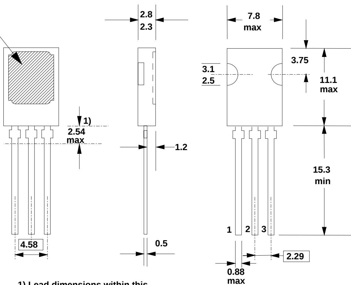
Fig.7. SOT82; pin 2 connected to mounting base.
