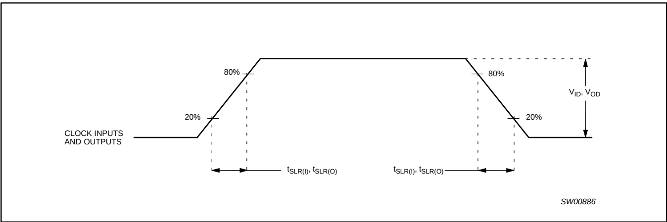
Figure 3. Input and output slew rates
