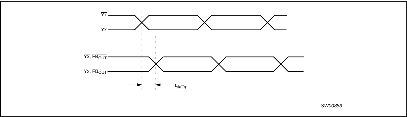
Figure 2. Output skew
