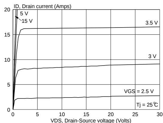
Fig.5. Typical output characteristics, T_j = 25\text{ °C} . I_D = f(V_{DS}) ; parameter V_{GS}
