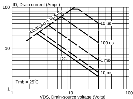
Fig.3. Safe operating area. T_{mb} = 25\text{ °C} I_D & I_{DM} = f(V_{DS}) ; I_{DM} single pulse; parameter t_p
