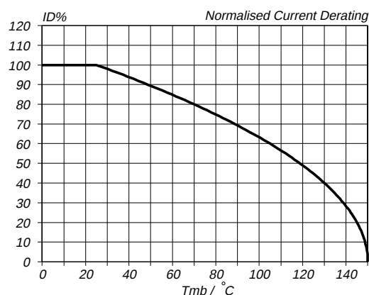
Fig.2. Normalised continuous drain current. ID\% = 100 \cdot I_D / I_{D\ 25^\circ\text{C}} = f(T_{mb}); \text{ conditions: } V_{GS} \geq 10\text{ V}
