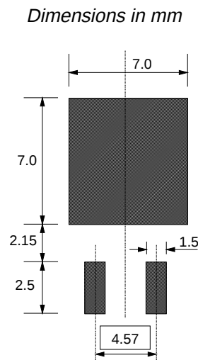
Fig.20. SOT428 : soldering pattern for surface mounting.
