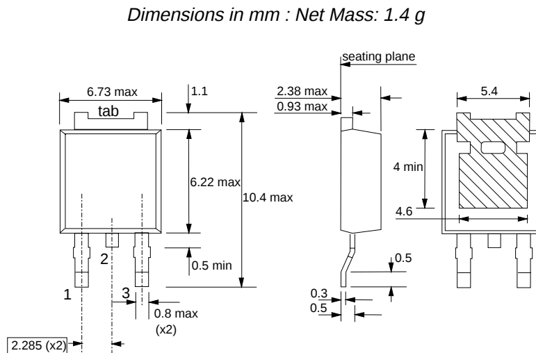
Fig.19. SOT428 : centre pin connected to mounting base.
