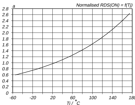
Fig. 9. Normalised drain-source on-state resistance. a = R_{DS(ON)}/R_{DS(ON)25^\circ\text{C}} = f(T_J) ; I_D = 3.3\text{ A} ; V_{GS} = 5\text{ V}
