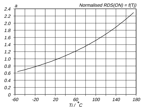
Fig.9. Normalised drain-source on-state resistance. a = R_{DS(ON)}/R_{DS(ON)25^\circ\text{C}} = f(T_J) ; I_D = 5.6 \text{ A} ; V_{GS} = 5 \text{ V}
