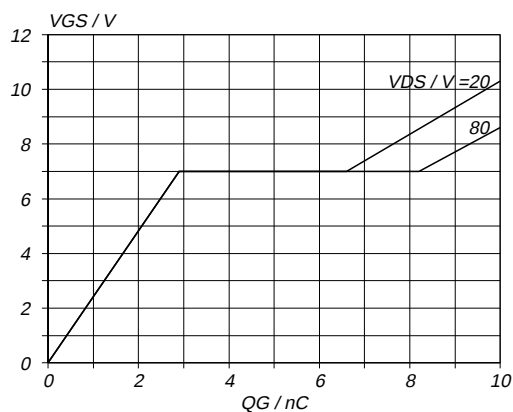
Fig.13. Typical turn-on gate-charge characteristics. V_{GS} = f(Q_G) ; conditions: I_D = 11 A; parameter V_{DS}
