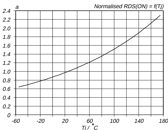
Fig.9. Normalised drain-source on-state resistance. a = R_{DS(ON)}/R_{DS(ON)25\text{ °C}} = f(T_j) ; I_D = 5.5 A; V_{GS} = 10 V
