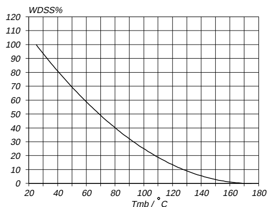
Fig.15. Normalised avalanche energy rating. W_{DSS}\% = f(T_{mb}) ; conditions: I_D = 11 A
