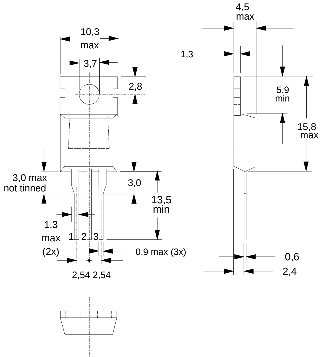
Fig.1. SOT78 (TO220AB); pin 2 connected to mounting base.
