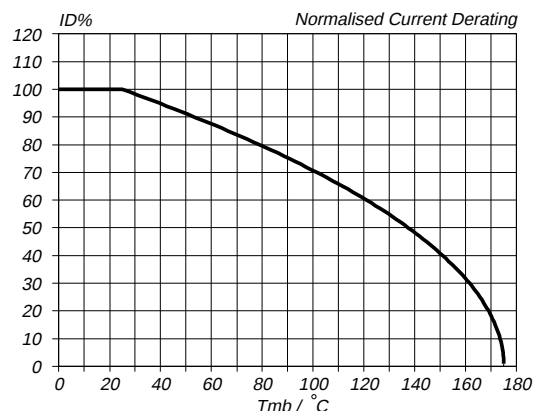
Fig.2. Normalised continuous drain current. ID\% = 100 \cdot I_D / I_{D\ 25^\circ\text{C}} = f(T_{mb}); \text{ conditions: } V_{GS} \geq 5\text{ V}
