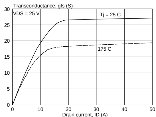
Fig.8. Typical transconductance g_{fs} = f(I_D)
