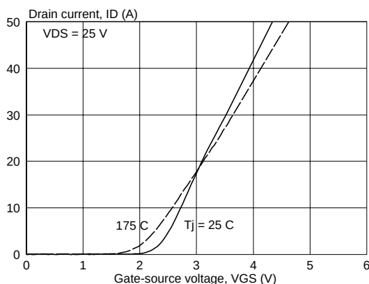
Fig.7. Typical transfer characteristics. I_D = f(V_{GS})
