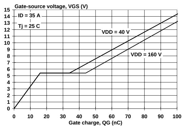
Fig.13. Typical turn-on gate-charge characteristics. V_{GS} = f(Q_G)
