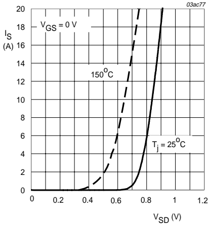
Fig 13. Source (diode forward) current as a function of source-drain (diode forward) voltage; typical values.
